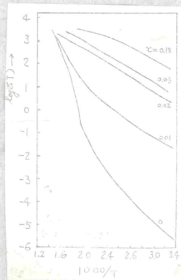
Fig. 2 \text{Li}_x\text{Ni}_{1-x}\text{O} at atmospheric pressure
